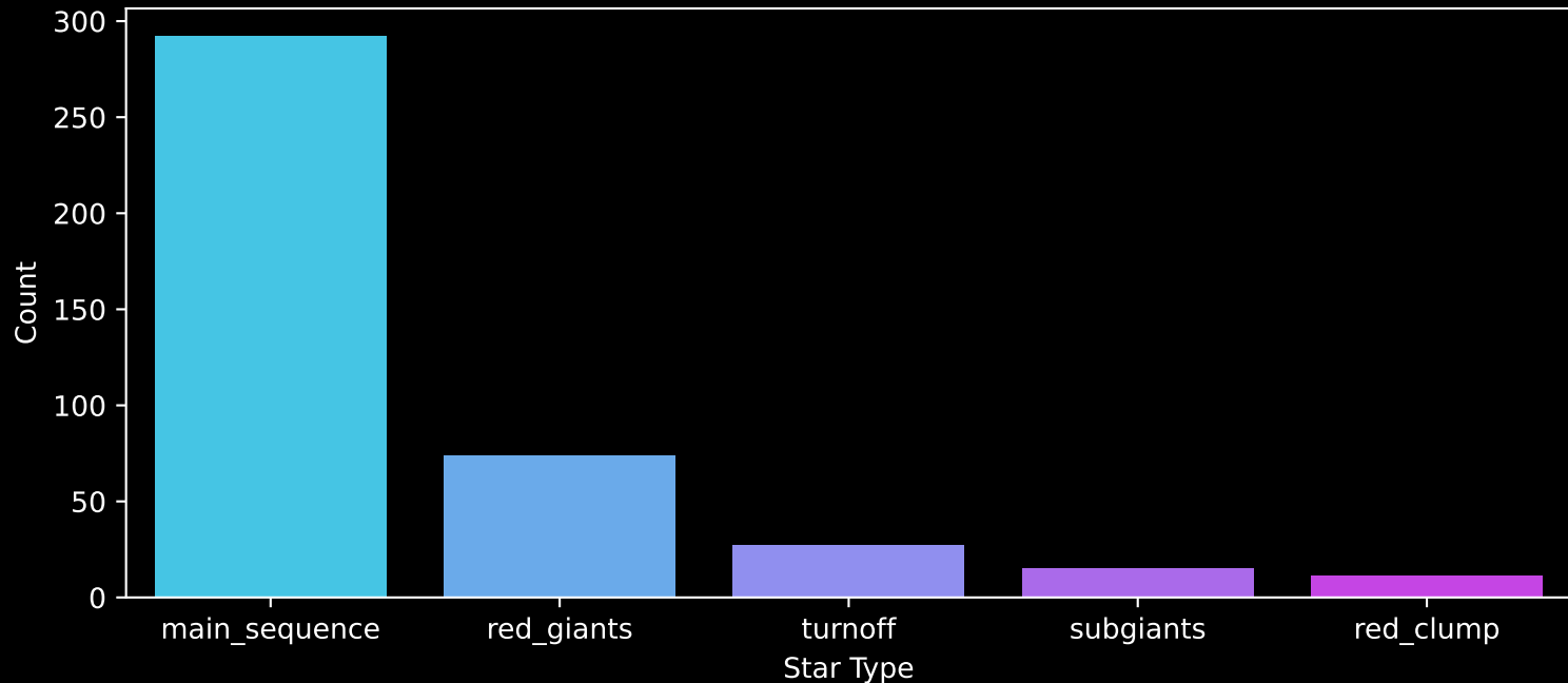
APOGEE DR17 Field: [000+75] Count plot of Star Type
