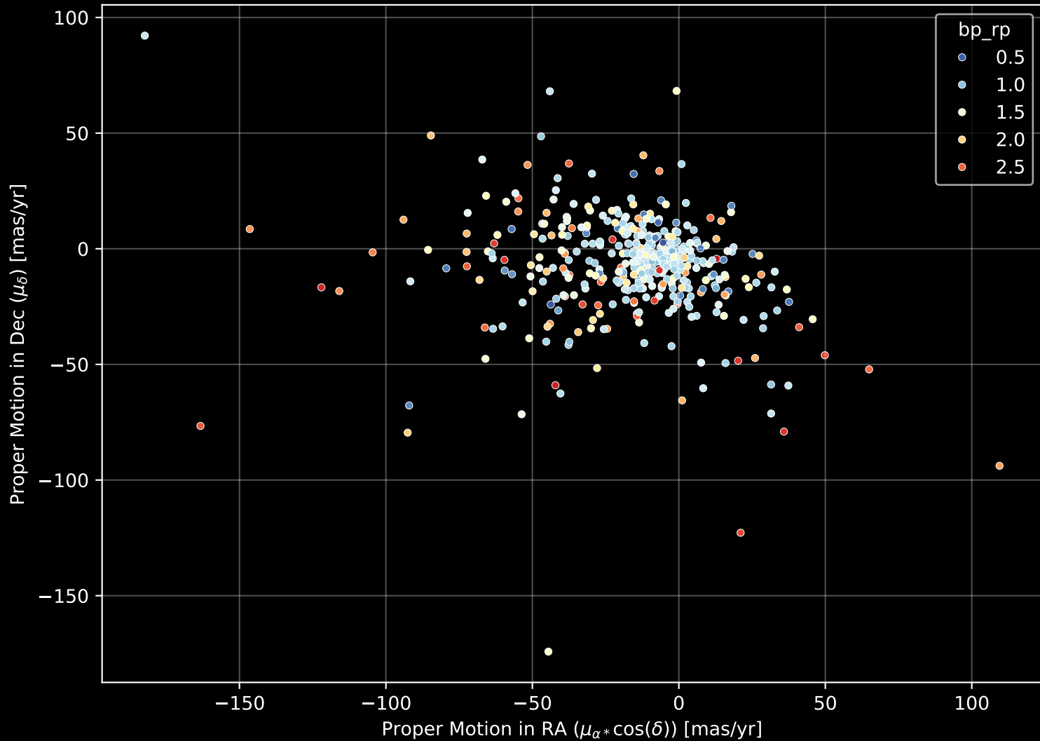
APOGEE DR17 Field: [000+75] Proper Motion Diagram (n= 419)
