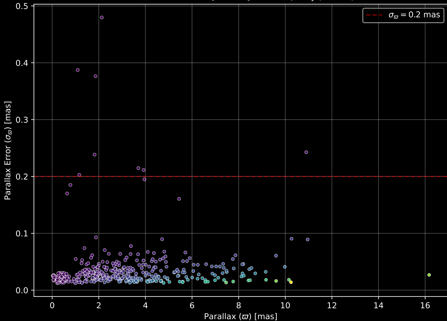
APOGEE DR17 Field: [000+75] Parallax Quality (n= 419)
