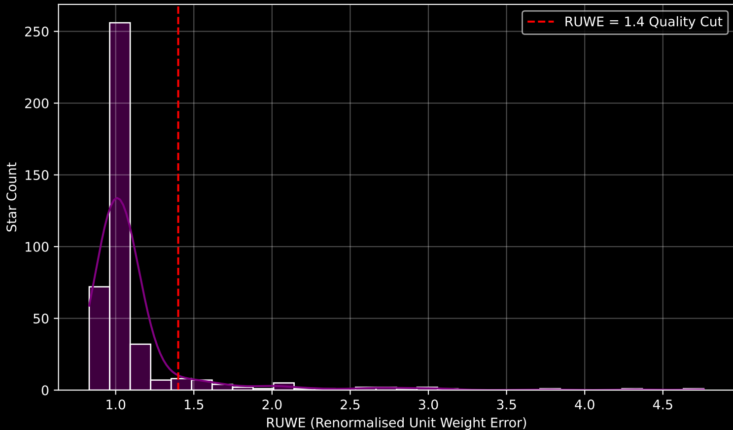
GAPOGEE DR17 Field [000+75] RUWE Distribution (n= 407)
