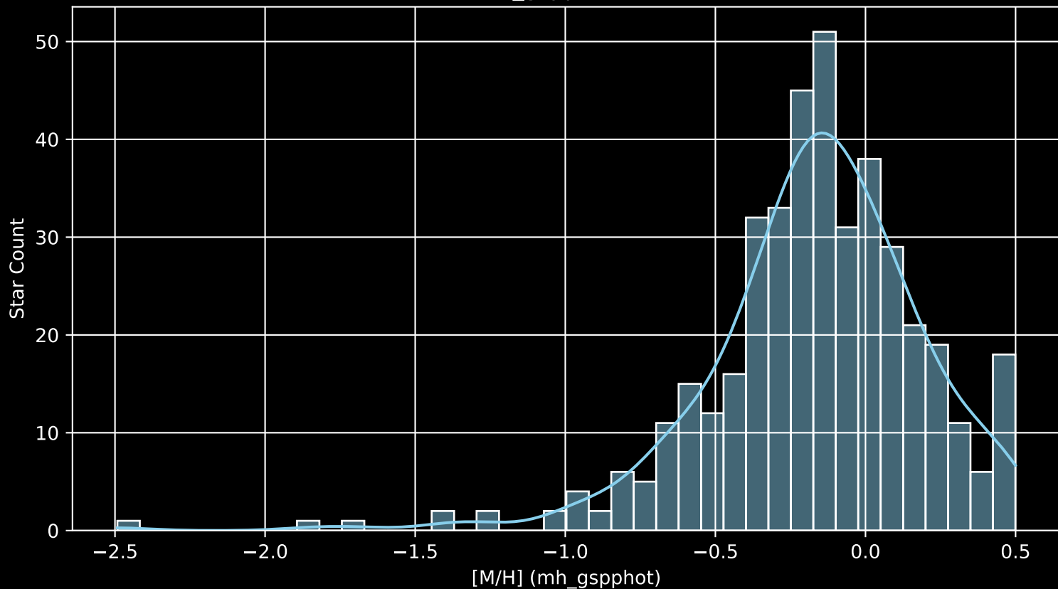
APOGEE DR17 Field: [000+75 [M/H] (mh_gspphot) (n= 414)
